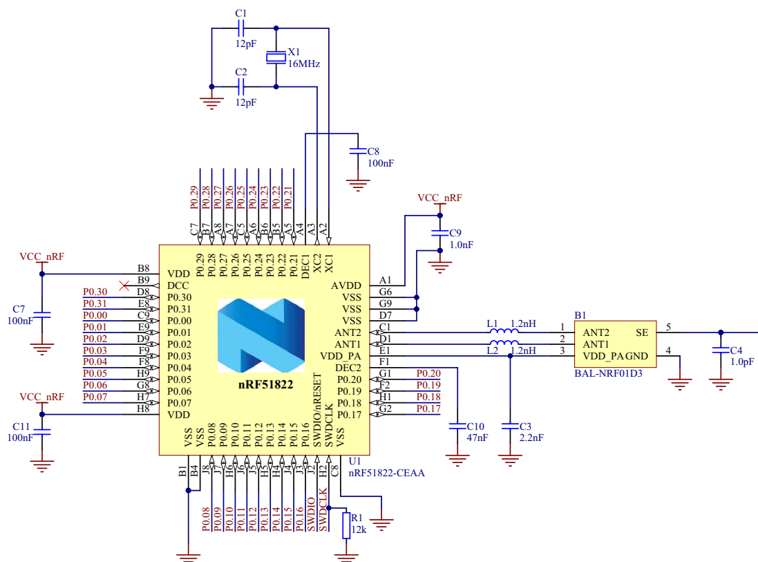
Figure 16 nRF51822 WLCSP with internal LDO regulator
