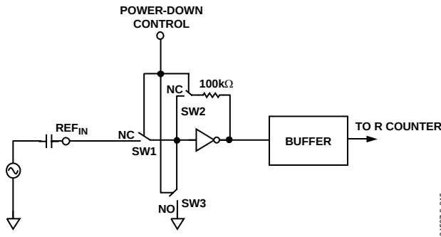
Figure 9. Reference Input Stage
