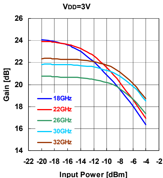
GAIN vs. INPUT POWER
