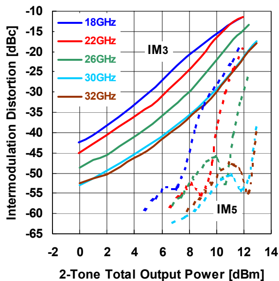
IMD PERFORMANCE vs. TOTAL OUTPUT POWER
