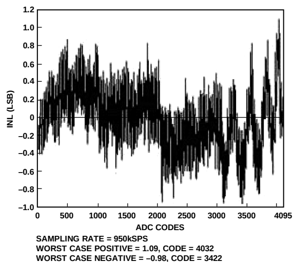
Figure 12. Typical INL, f_{ADC} = 950 kSPS, External 1.0 V Reference Used
