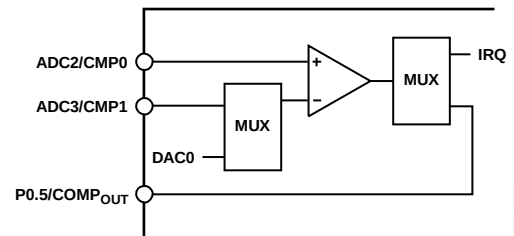
Figure 34. Comparator
