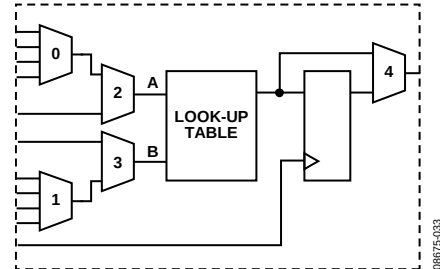
Figure 39. PLA Element
