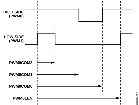
Figure 40. PWM Timing
