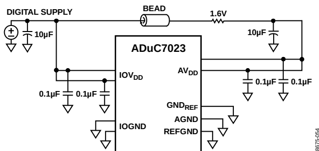
Figure 47. External Single Supply Connections
