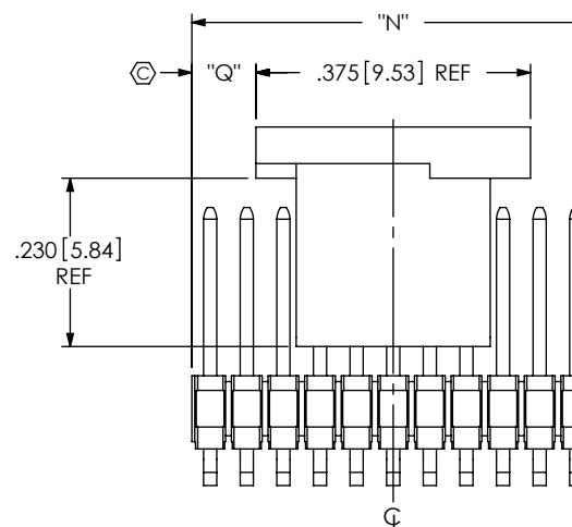
FIG 2 -A OPTION: ALIGNMENT PIN (DIFFERENT AS SHOWN, OTHERWISE SEE FIG 1)
