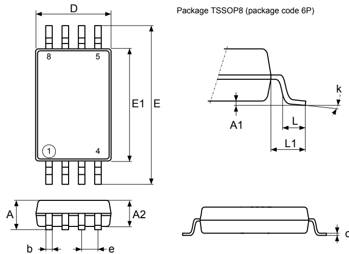
Figure 17. TSSOP8 – Outline
