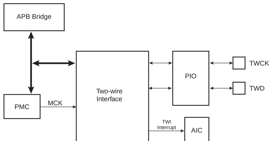
Figure 30-1. Block Diagram
