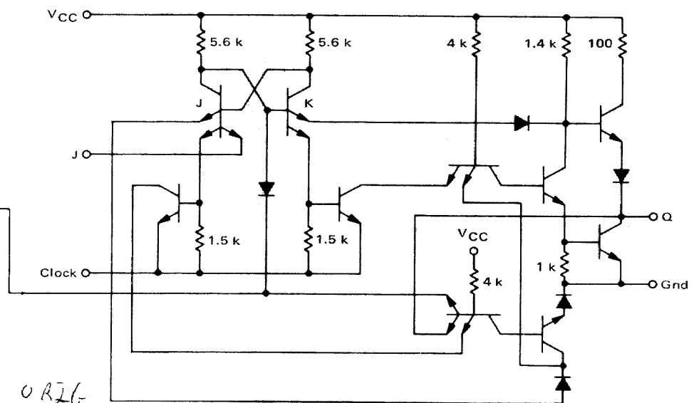
TYPICAL FLIP-FLOP
