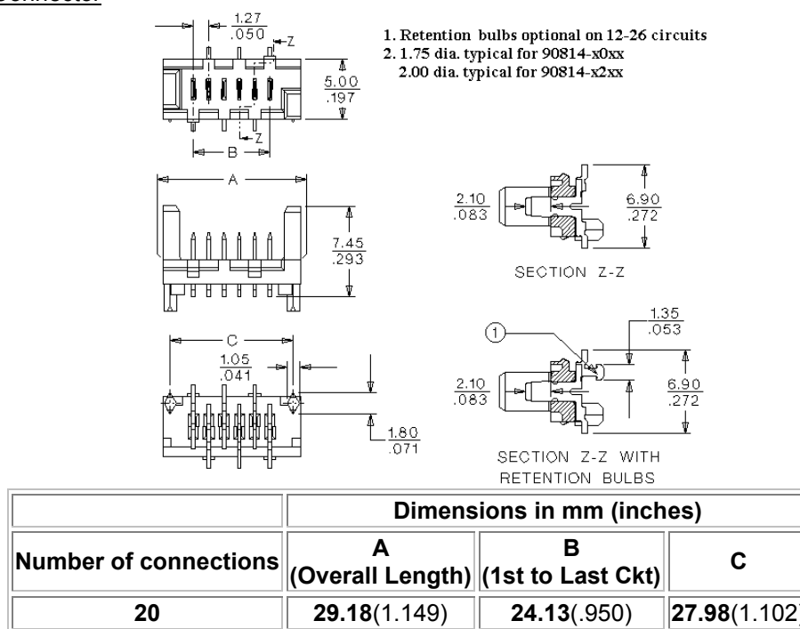
Figure 1. Picoflex Connector
