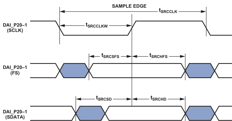
Figure 26. SRC Serial Input Port Timing
