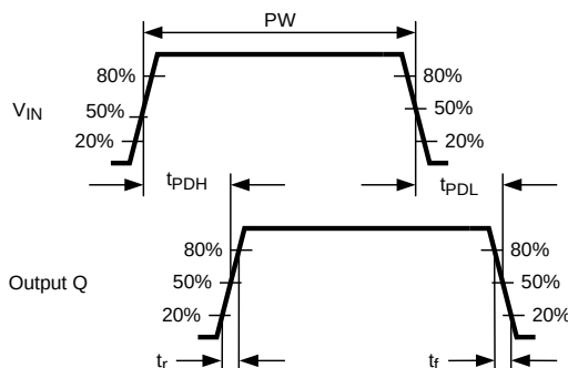
Figure 26. Propagation Delay
