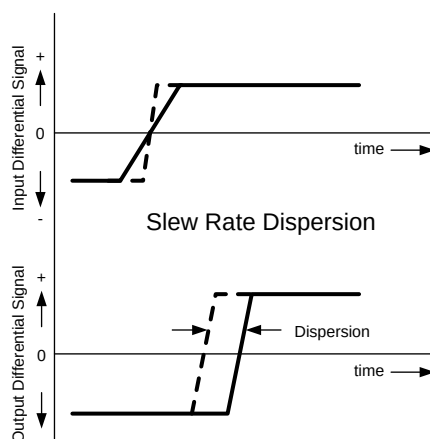
Figure 29. Slew Rate Dispersion
