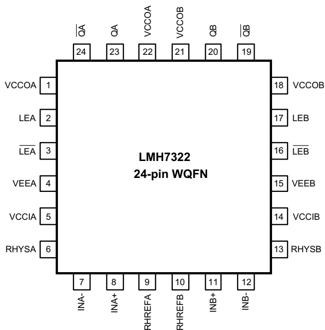
Figure 3. Footprint
