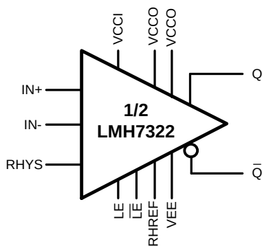
Figure 2. Schematic
