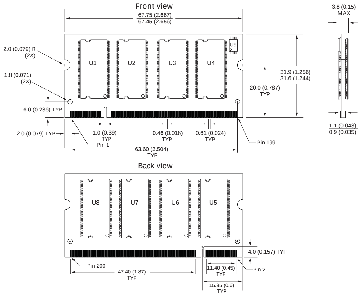
Figure 3: 200-Pin DDR SODIMM
