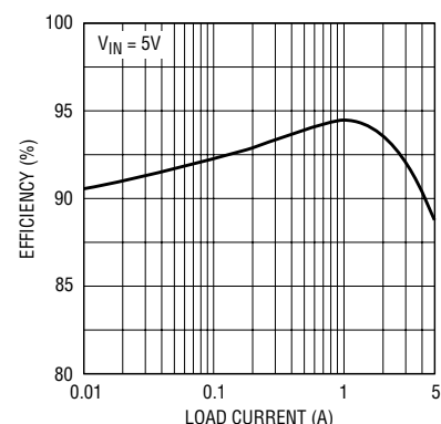
LTC1266-3.3 Efficiency
