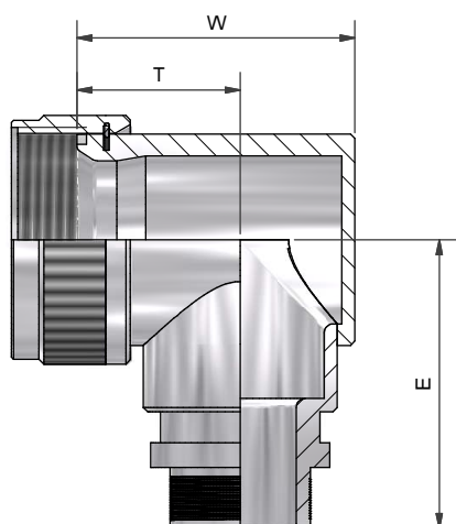
90° BACKSHELL - TYPE 1
