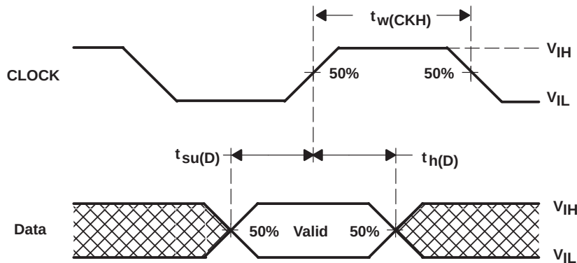
Figure 1. Input Timing
