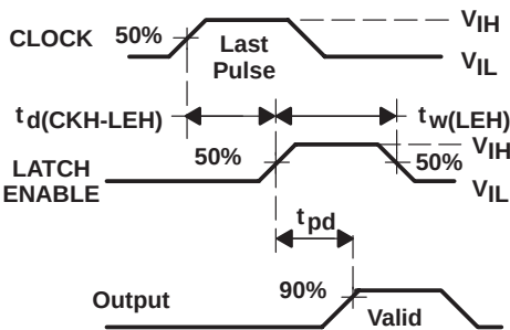
Figure 2. Output Switching Times
