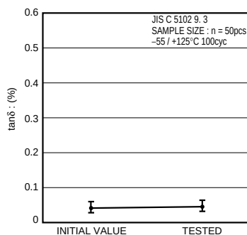
Fig.8 tanδ
