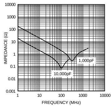
Fig.4 Impedance-frequency characteristics
