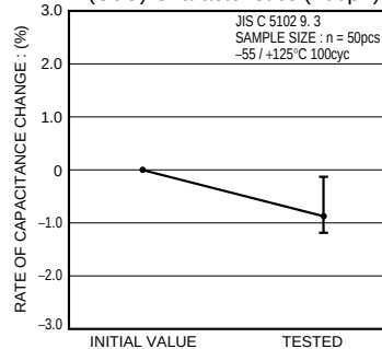
A (C0G) Characteristics (100pF)
