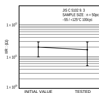
Fig.12 Insulation resistance
