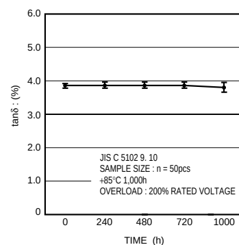
Fig.23 \tan\delta
