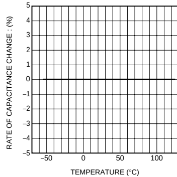
Fig.1 Capacitance-temperature characteristics
