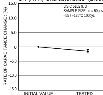
CN (X7R) Characteristics (1,000pF)
