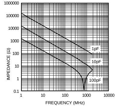
Fig.2 Impedance-frequency characteristics
