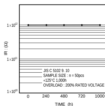
Fig.18 Insulation resistance
