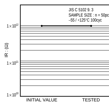
Fig.9 Insulation resistance
