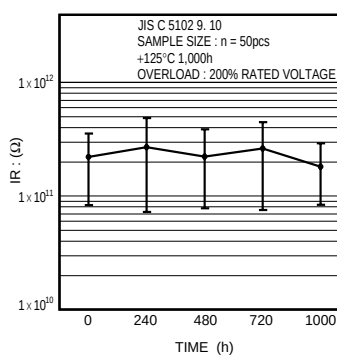
Fig.21 Insulation resistance
