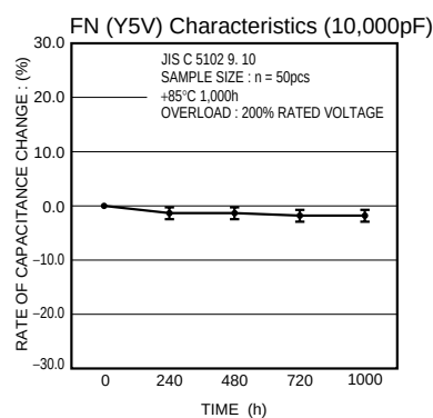
Fig.22 Rate of capacitance change
