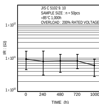
Fig.24 Insulation resistance
