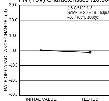
FN (Y5V) Characteristics (10,000pF)
