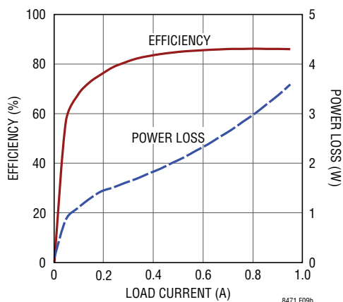
Figure 9b. Efficiency and Power Loss ( V_{CC} = 18V , Load from V_{OUT1} to V_{OUT2} )
