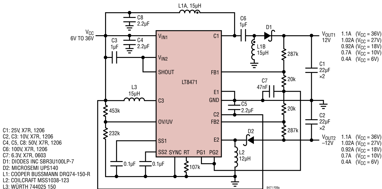
Figure 9a. Tracking \pm 12V Supplies from 6V to 36V Input at 800kHz
