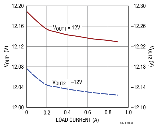
Figure 9c. 12V and -12V Outputs vs Load Current ( V_{CC} = 18V , Load from V_{OUT1} to V_{OUT2} )
