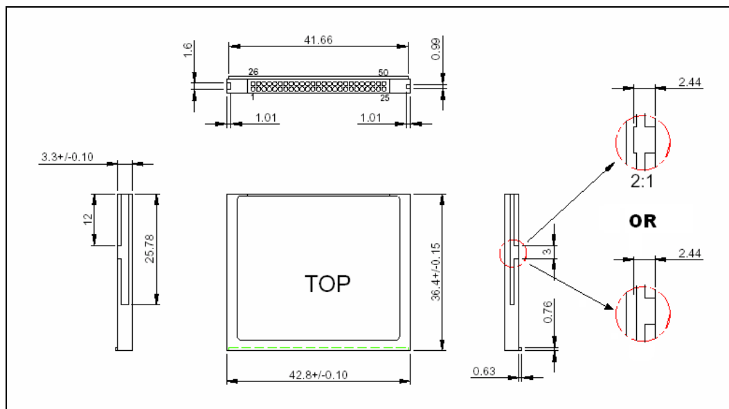
Figure 2-1. Physical Dimensions
