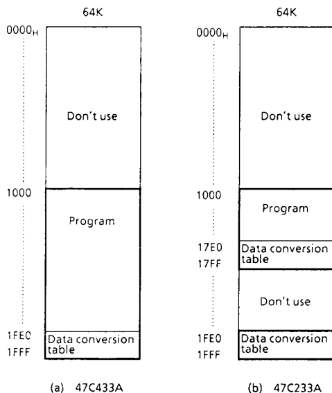
Figure 1. Program area
