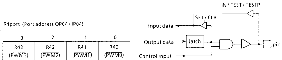
Figure 2-1. Port R4
