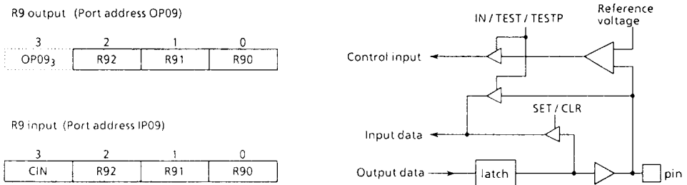
Figure 2-3. Port R9
