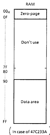
Figure 2. RAM addressing
