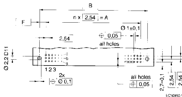
Mounting Holes (component side) for Printed Circuits. (For connectors with soldering pins angled at 90°.)
