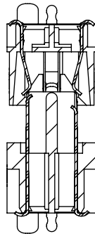
SECTION "F"-"F"
