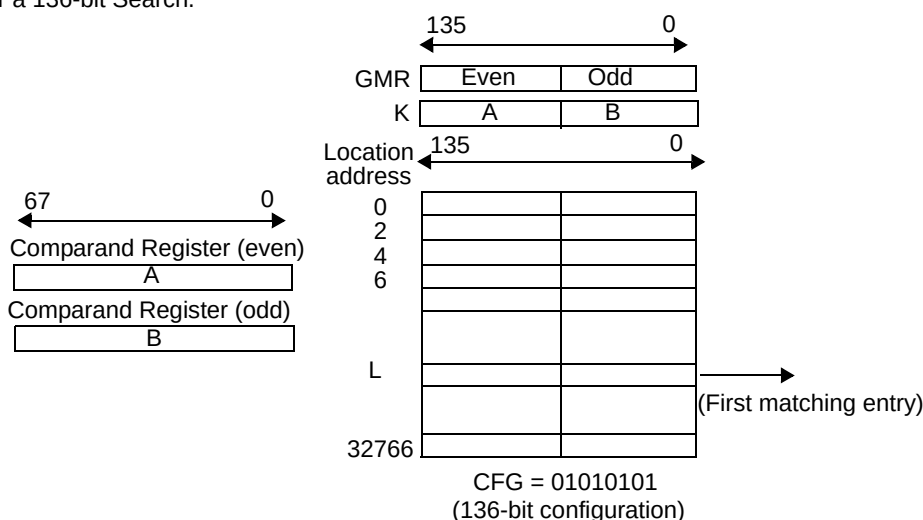
The Search command is a pipelined operation that executes searches at half the rate of the frequency of CLK2X for 136-bit searches in ×136-configured tables. The latency of SADR, CE_L, ALE_L, WE_L, SSV, and SSF from the 136-bit Search command cycle (two CLK2X cycles) is shown in Table 10-18 .
