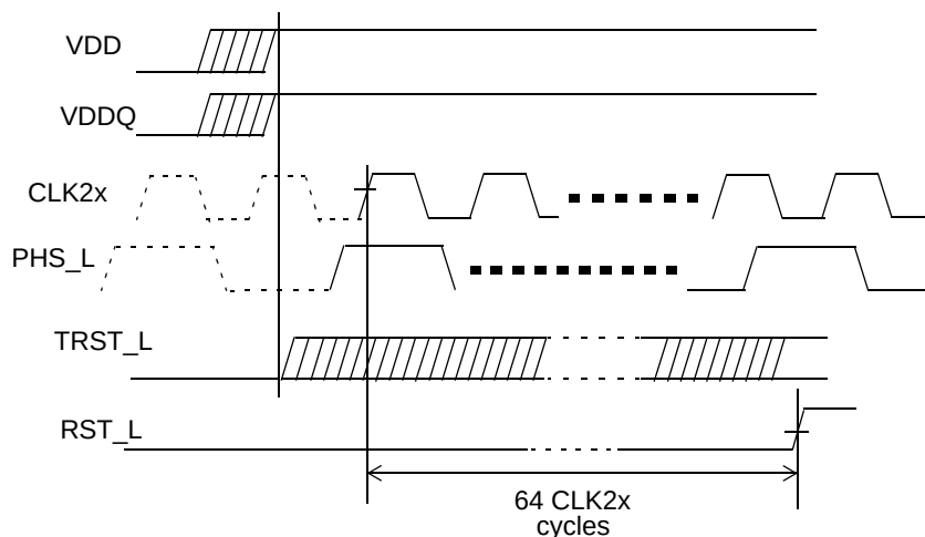
Figure 13-1. Power-up Sequence
