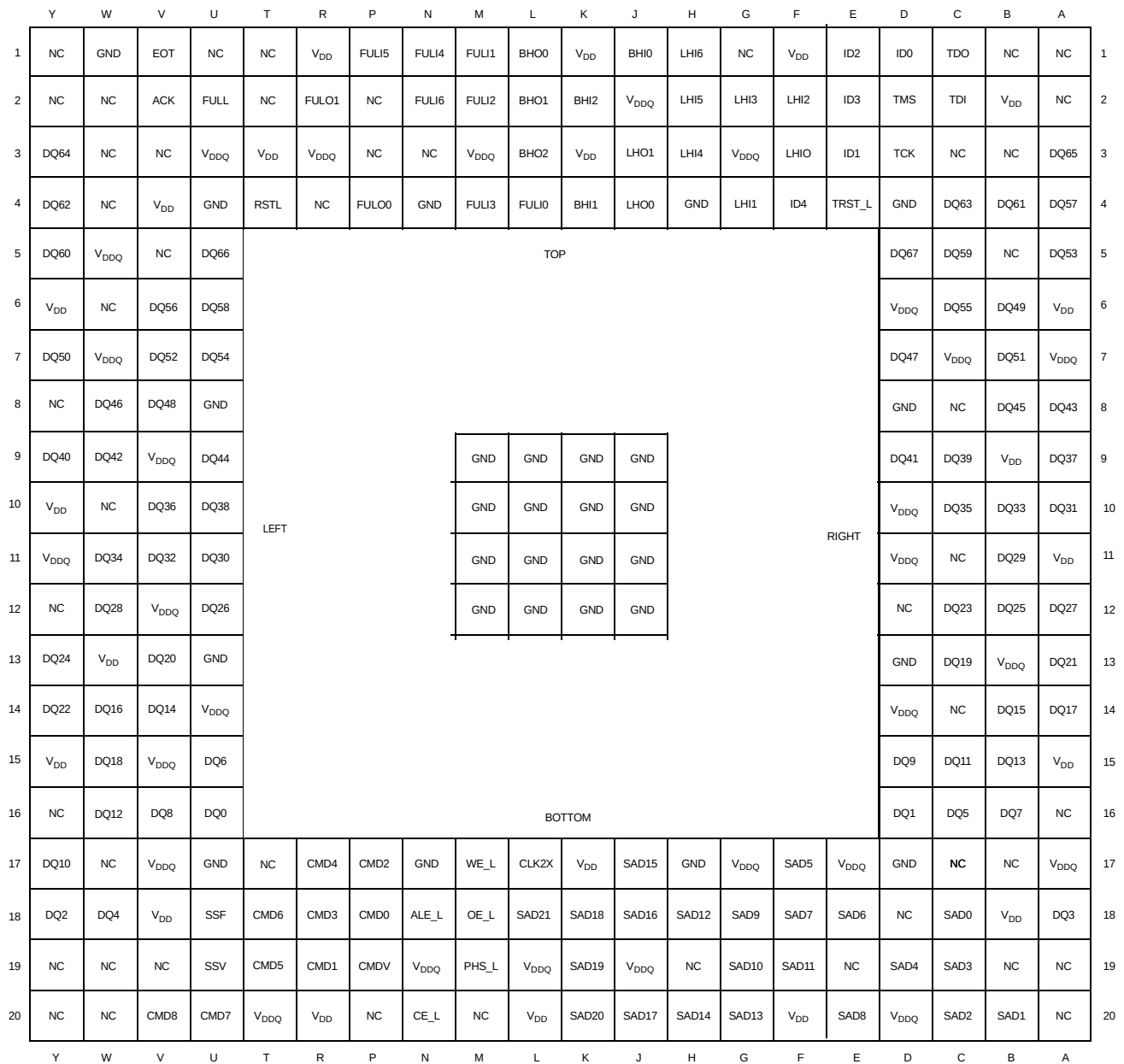
Figure 18-1. Pinout Diagram
