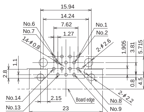
DX10LM1-14SE(50) DX10LM2-14SE(50)
