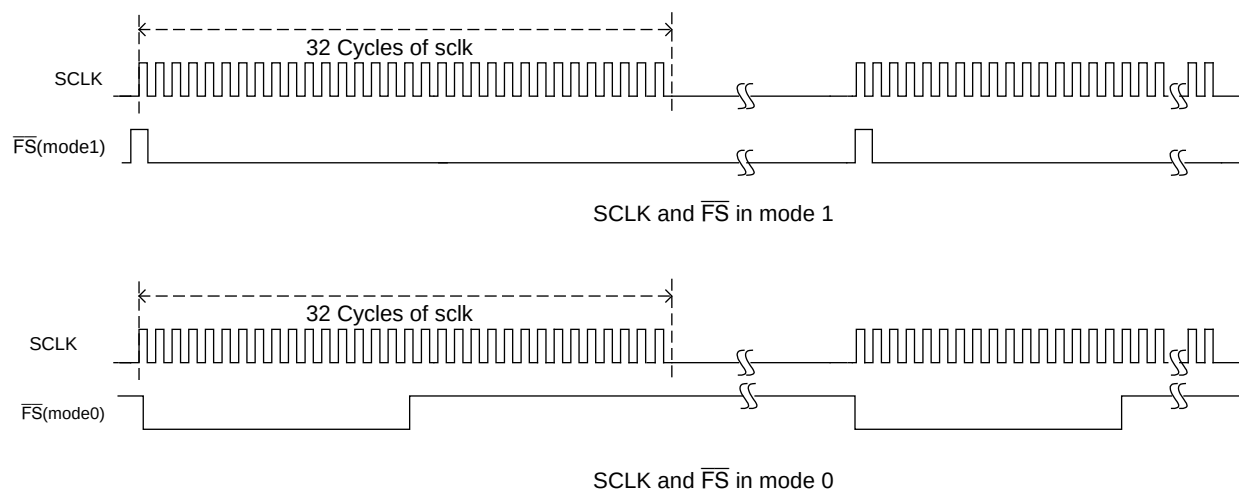
Figure 1: Effect of the TYPE (FS mode) pin on \overline{FS} with SckMode = 0
