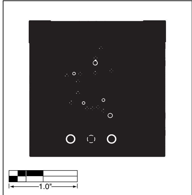
Figure 8. MAX9993 EV Kit PC Board Layout—Bottom Layer Metal
