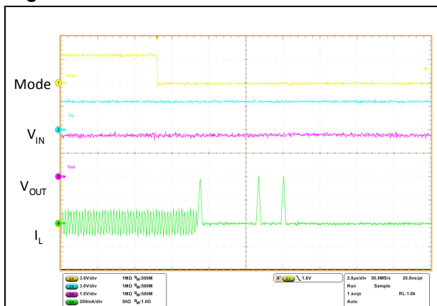
Figure 13. Mode transition PWM to PFM
