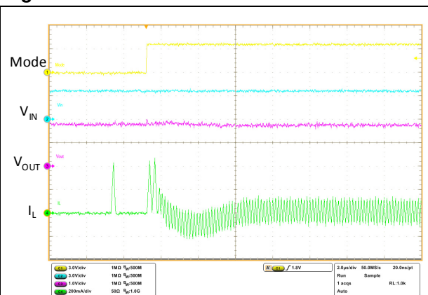
Figure 12. Mode transition PFM to PWM
