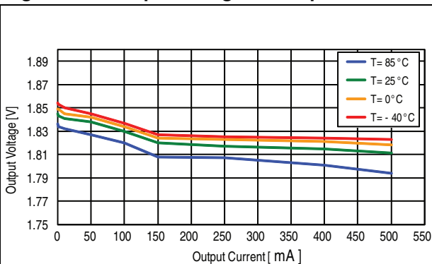
Figure 10. Output voltage vs. output current
