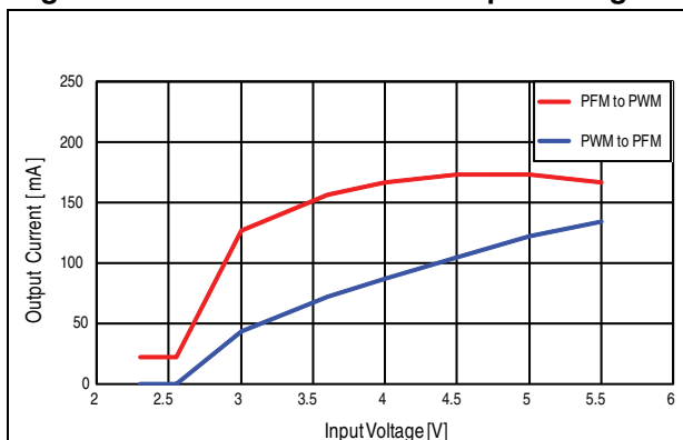
Figure 11. Mode transition vs. input voltage
