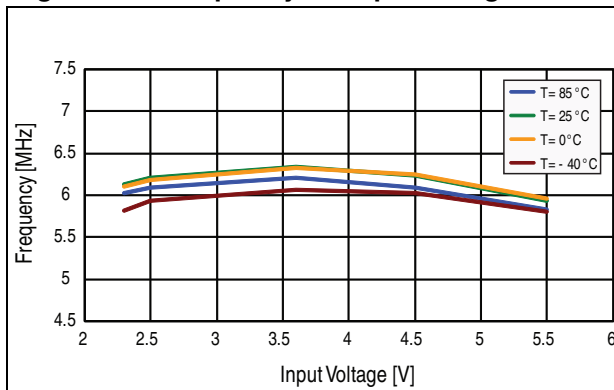
Figure 9. Frequency vs. input voltage
