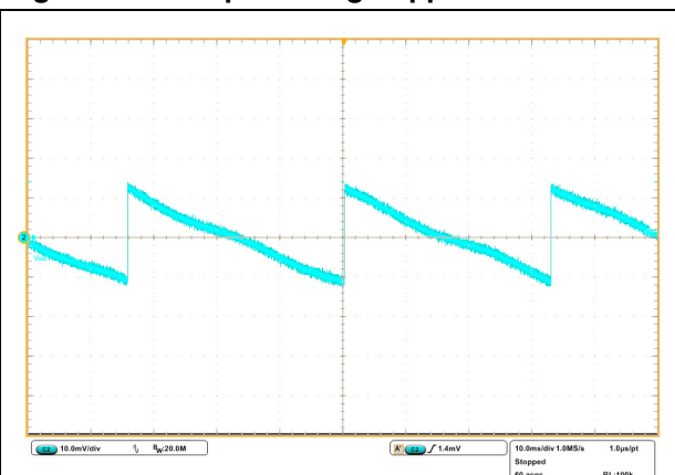
Figure 14. Output voltage ripple
