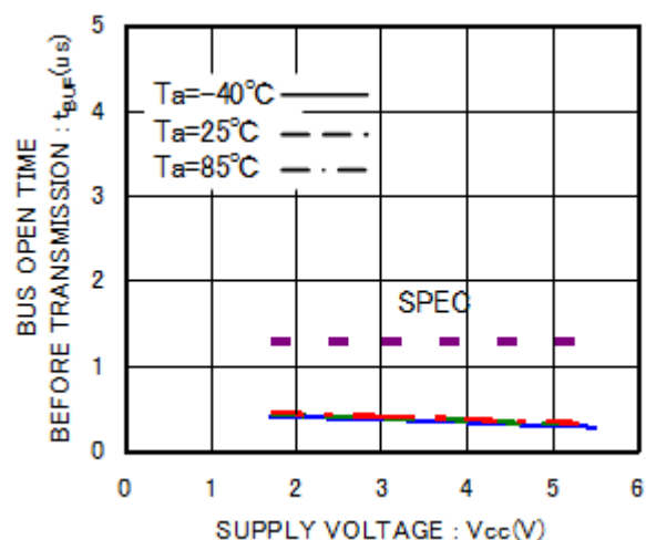
Figure 22. BUS open time before transmission t_{BUF}
