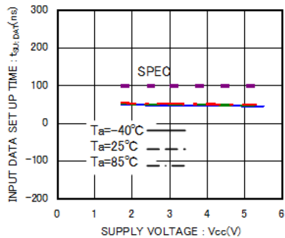
Figure 18. Input Data Setup Time t_{SU:DAT} (HIGH)
