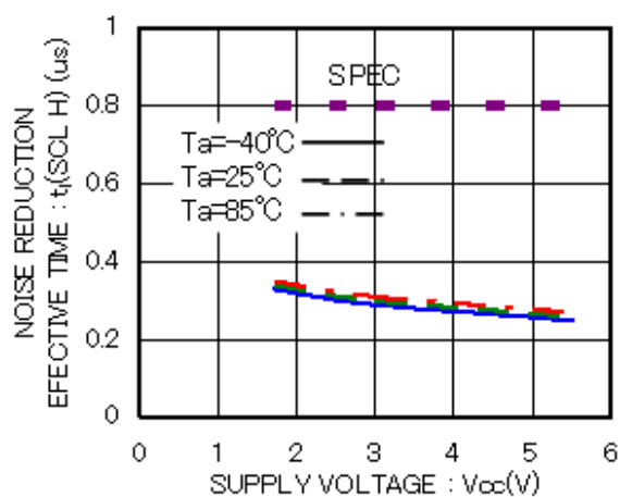
Figure 24. Noise reduction effective time t_i(SCL H)
