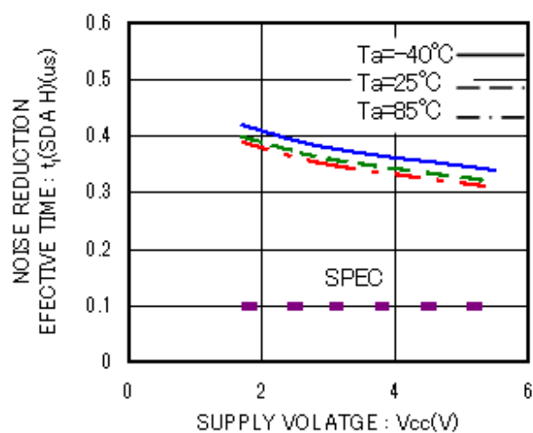
Figure 26. Noise reduction effective time t_i(\text{SDA H})
