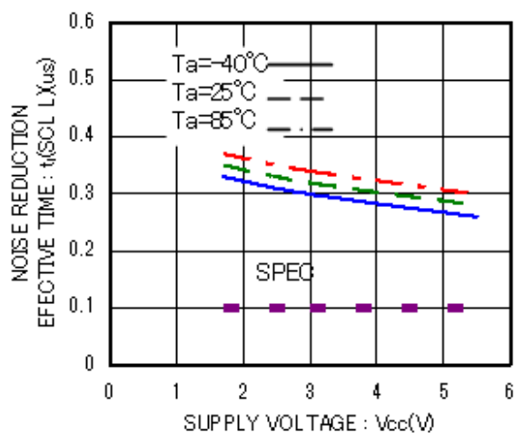
Figure 25. Noise reduction effective time t_i(SCL L)
