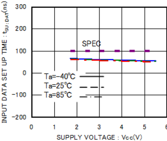
Figure 19. Input Data Setup Time t_{SU:DAT} (LOW)
