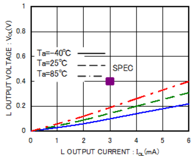
Figure 5. 'L' output voltage V_{OL} - I_{OL} ( V_{CC} = 2.5\text{V} )
