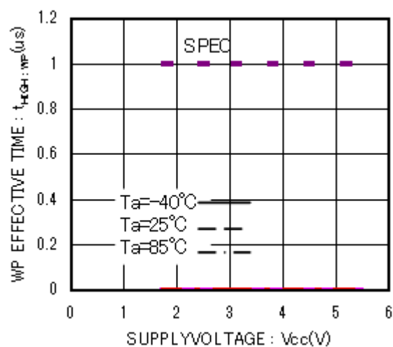
Figure 29. WP effective time t_{HIGH:WP}
