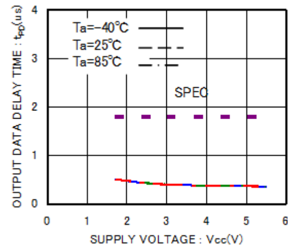
Figure 20. "L" Data output delay time t_{PD0}
