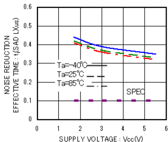
Figure 27. Noise reduction effective time t_i(\text{SDA L})
