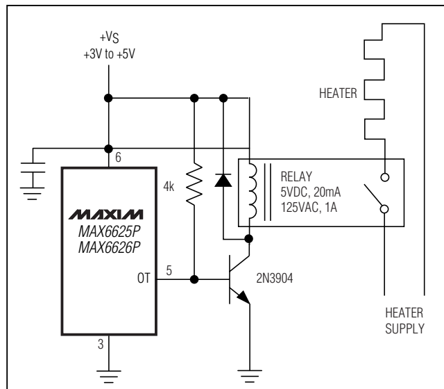
Figure 8. Simple Thermostat
