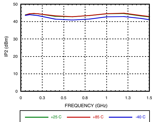
Low Frequency OIP2 vs. Temperature @ Pout/tone = +16dBm
