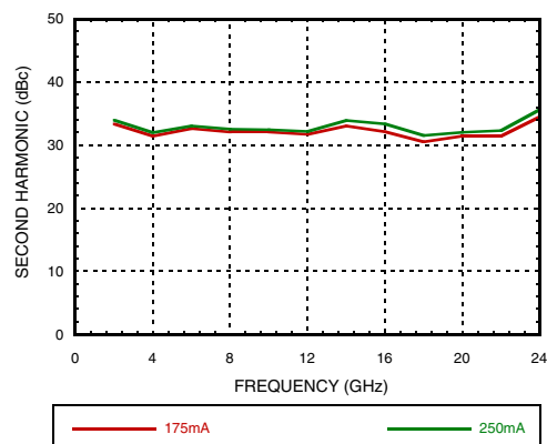
Second Harmonics vs. Idd @ Pout = +14dBm
