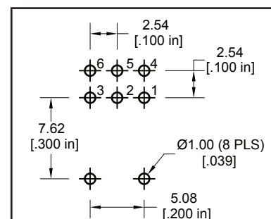
DOUBLE POLE PCB LAYOUT
