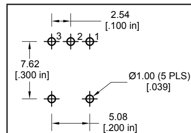
SINGLE POLE PCB LAYOUT
