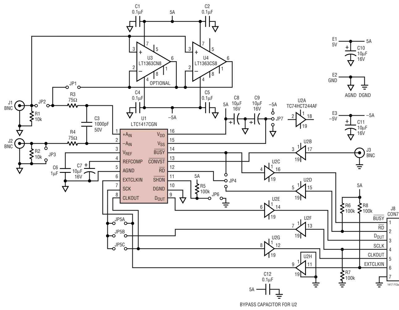
Figure 13a. Suggested Evaluation Circuit Schematic
