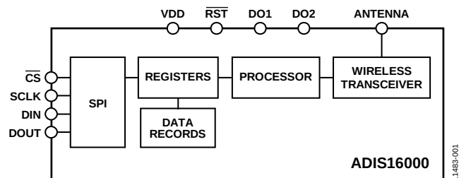
Figure 1. ADIS16000 Block Diagram
