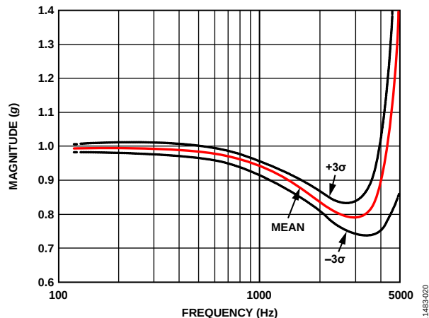
Figure 21. Magnitude/Frequency Response
