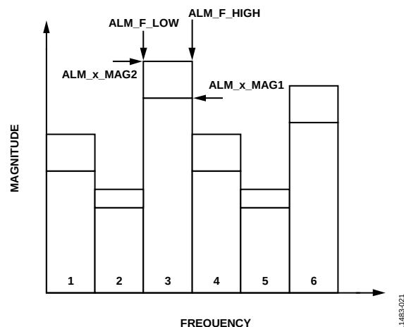
Figure 22. Spectral Band Alarm Setting Example, ALM_PNTR = 0x03
