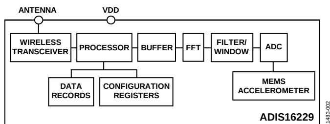
Figure 2. ADIS16229 Block Diagram
