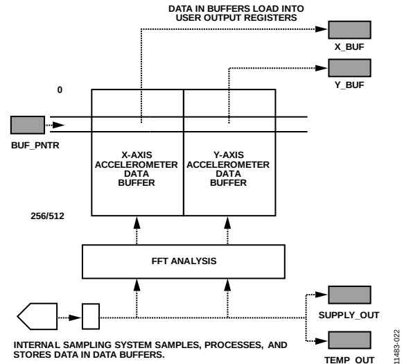
Figure 23. Data Buffer Structure and Operation
