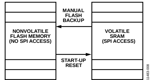
Figure 11. SRAM and Flash Memory Diagram
