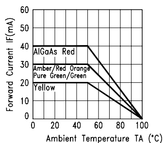
Fig.4 FORWARD CURRENT DERATING CURVE
