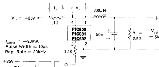
Figure 1. PIC600, 601, 602 Switching Speed Circuit
