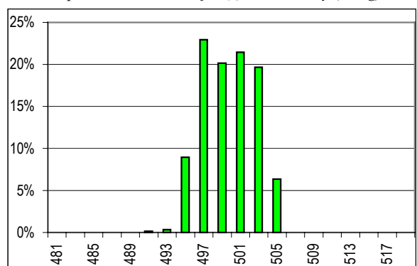
Graph 8. Distribution of AOUTY Sensitivity (mV/g)
