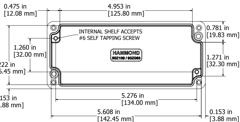
Top View Looking Inside Box
