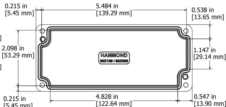
View Looking Inside Lid
