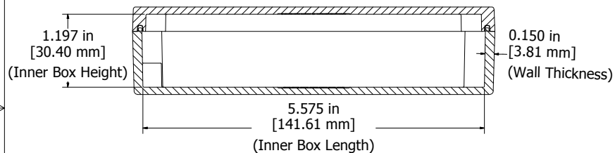
SECTION B-B Side View of Assembly
