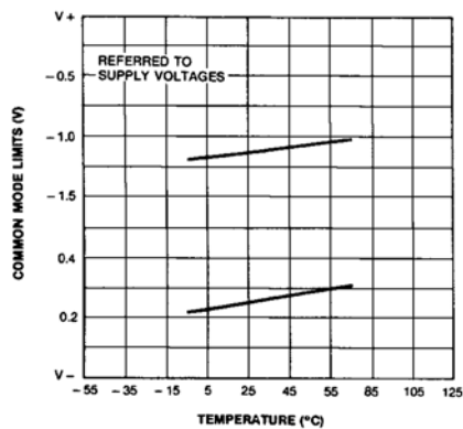
FIGURE 5. Common Mode Limits vs. Temperature
