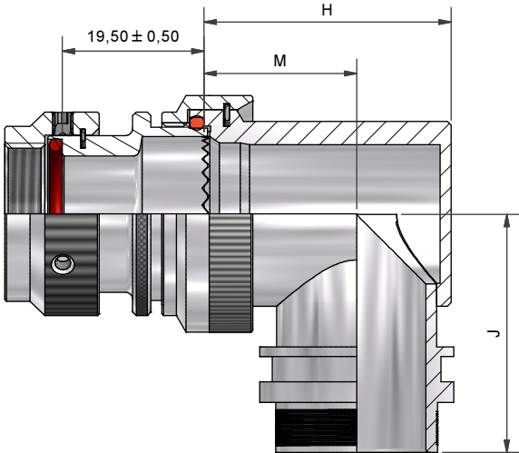
90° BACKSHELL - TYPE 2
