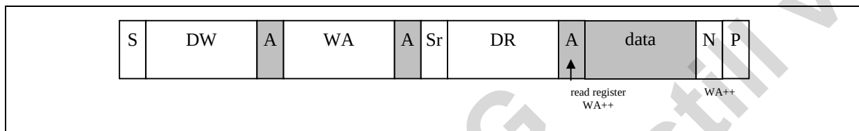
Figure 53. I^2C Random-Read:
