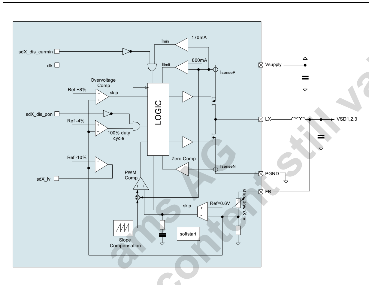
Figure 27. Step Down DC/DC Converter Block diagram
