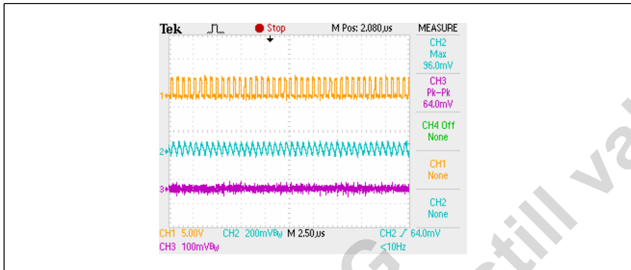
Figure 28. sdX_dis_curmin=1 operation
