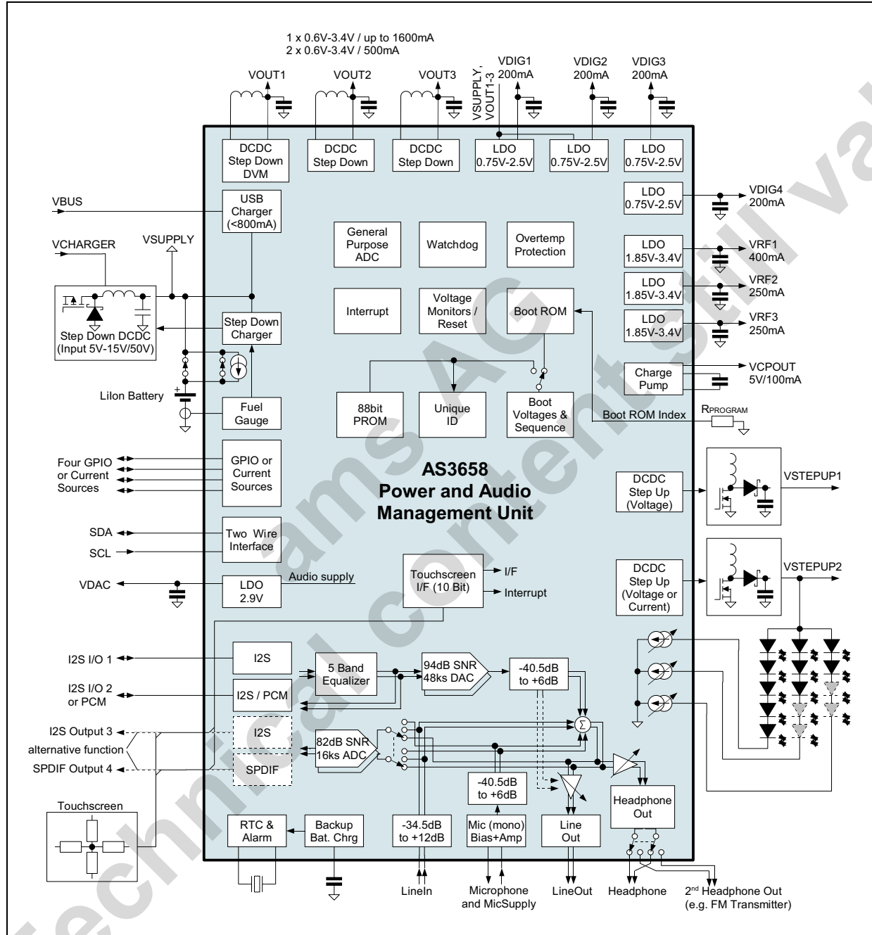
Figure 1. Blockdiagram AS3658
