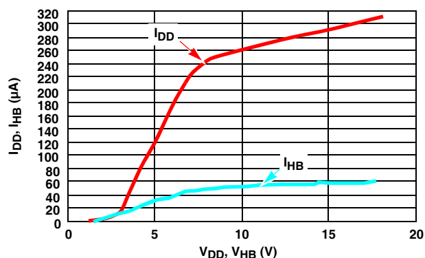
FIGURE 20. ISL2111 QUIESCENT CURRENT vs VOLTAGE
