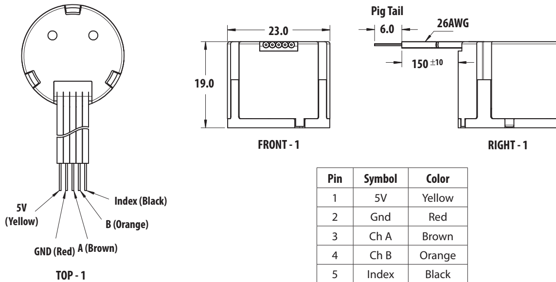
Figure 4. Electrical Connections
