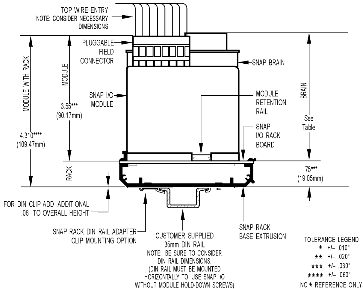
SNAP Analog Module Mounted on a SNAP Rack
