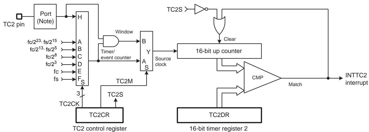
Figure 9-1 Timer/Counter2 (TC2)
