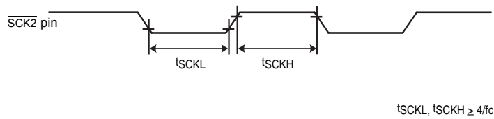
Figure 15-3 External Clock
