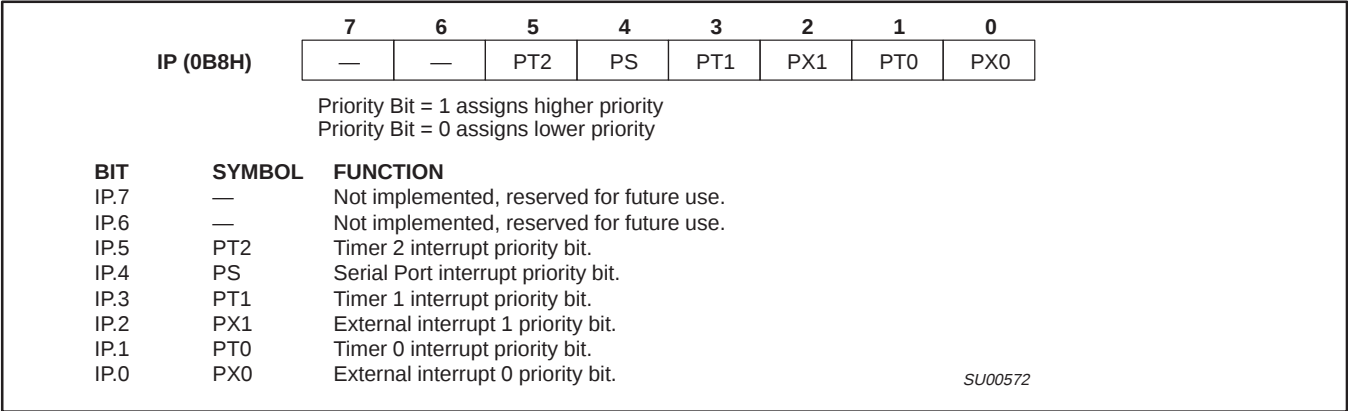
Figure 11. IP Registers
