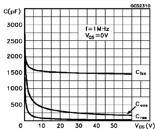
Capacitance Variations
