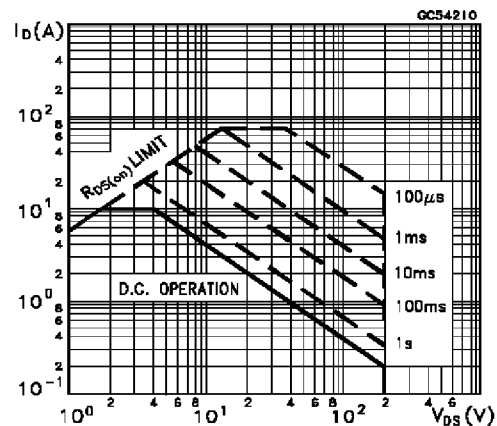
Safe Operating Area for ISOWATT220
