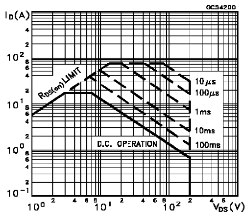
Safe Operating Area for TO-220
