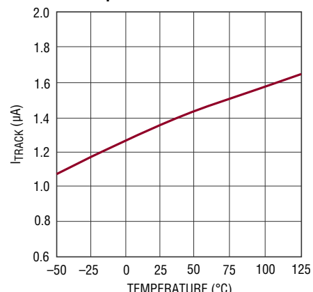
Track Pull-Up Current vs Temperature
