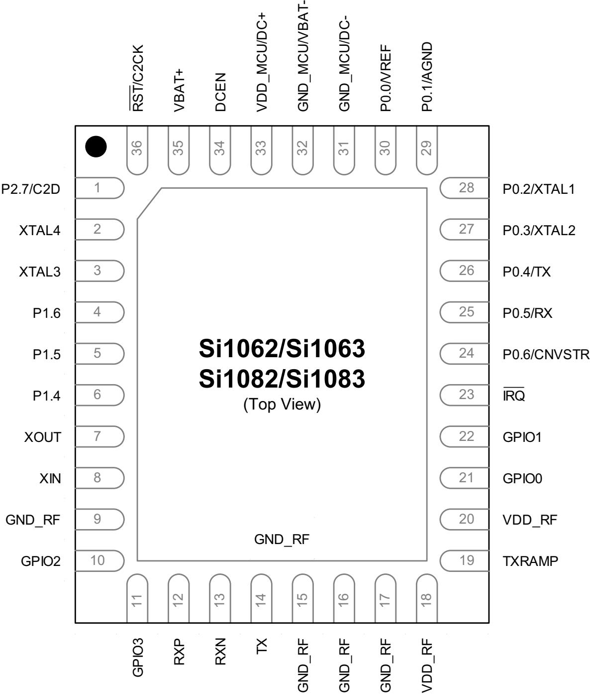
Figure 3.2. Si1062/3, Si1082/3-A-GM Pinout Diagram (Top View)
