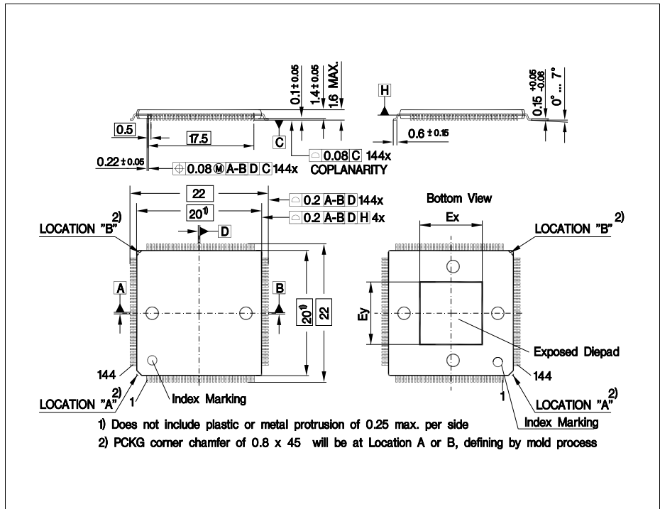
Figure 30 PG-LQFP-144-16I-23 (Plastic Green Thin Quad Flat Package)
