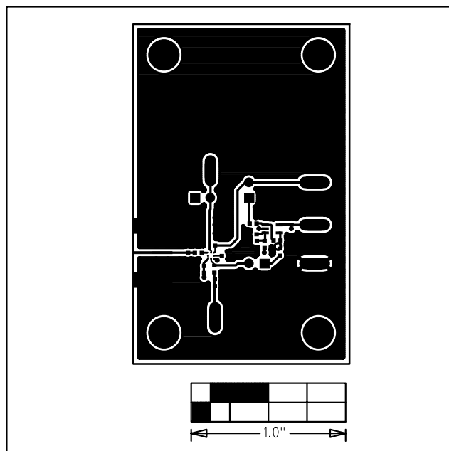
Figure 3. MAX4001 EV Kit PC Board Layout—Component Side
