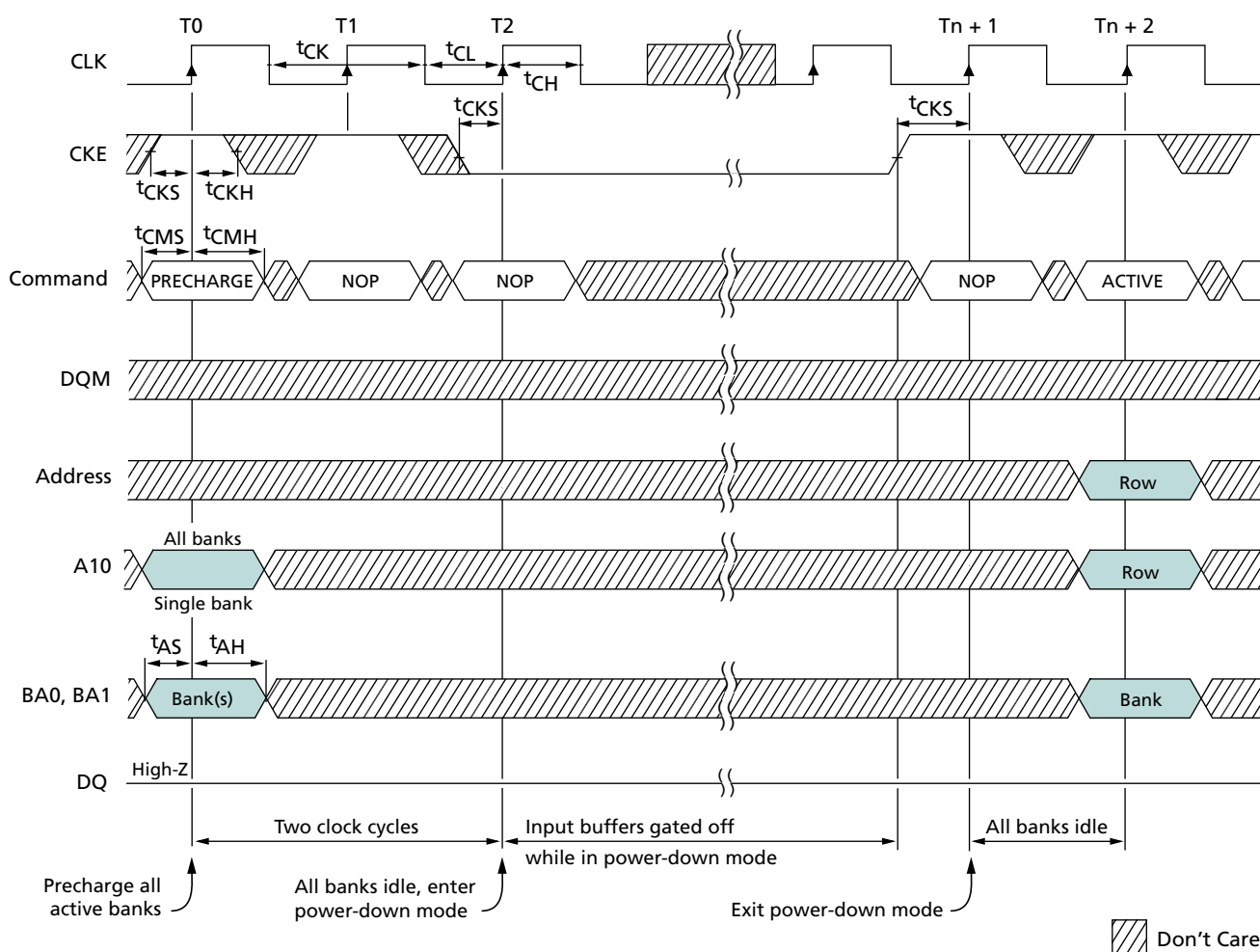
Figure 48: Power-Down Mode
